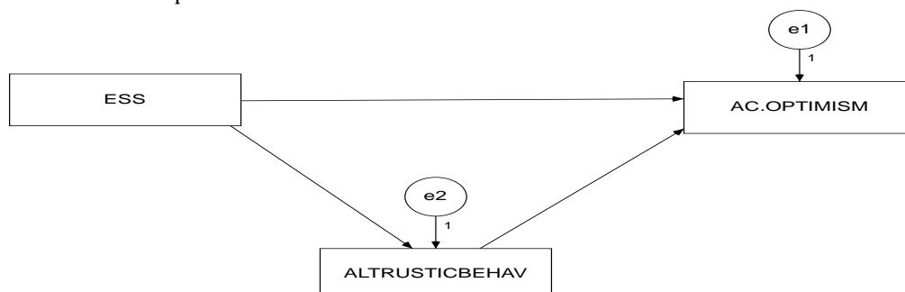
Figure 2. Theoretical model
